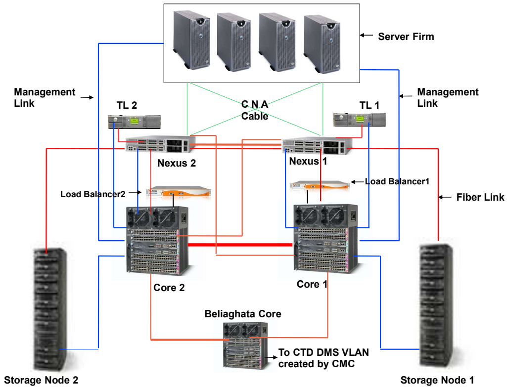
Network Diagram for WBCOMTAX Project
